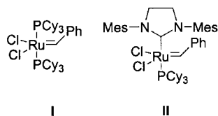
Figure 1. First ( I ) and second ( II ) generation Grubbs' catalyst
