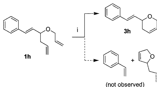
Scheme 3. i , CH 2 Cl 2 , 20 °C, I (5 mol %) (90%)
