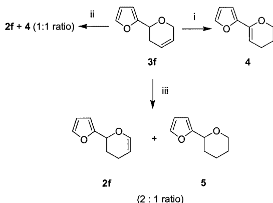
Scheme 4. i , KO t Bu, DMSO, 100 °C (75%); ii , [RhCl(PPh 3 ) 3 ] (5 mol %), DBU (1.5 equiv.), EtOH, 78 °C (90% of 2f and 4 ); iii , [RuCl 2 (PPh 3 ) 3 ] (2.6 mol %), NaBH 4 (25 mol %), MeOH, 65 °C (40% of 2f and 21% of 5 )
